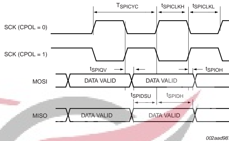
Fig 25. SPI master timing (CPHA = 0)
